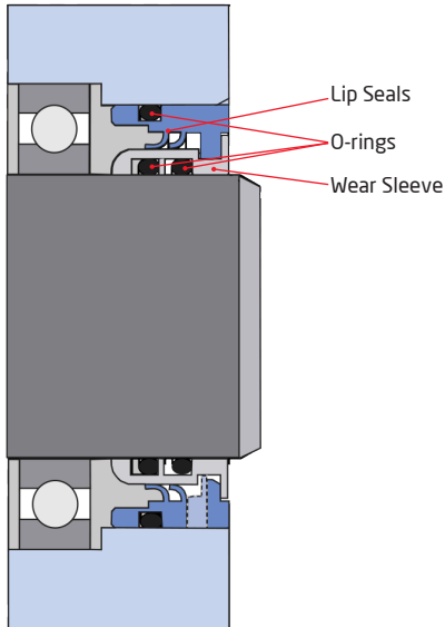
Non-Flanged
