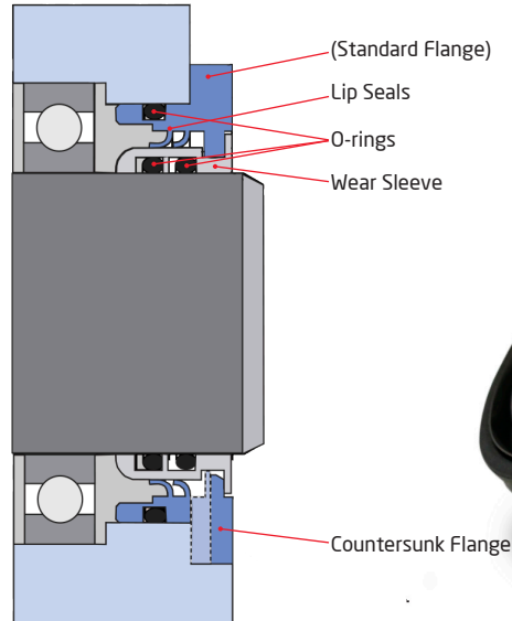
Flanged
